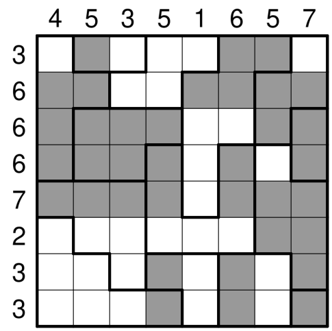
8.8 Kippliges Aquarium 2
