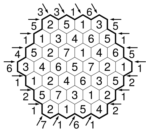
2.6 HexRooms
