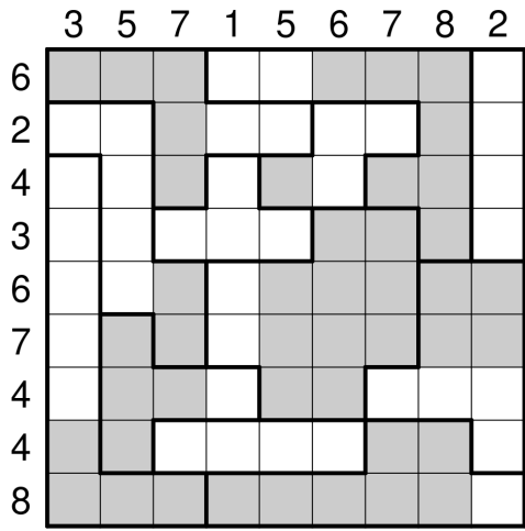
8.7 Kippliges Aquarium 1
