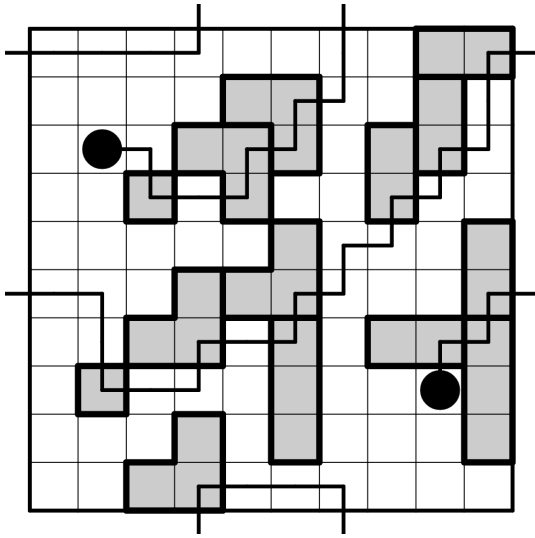
4.7 Toroidal POM
