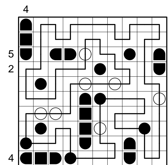
4.6 Masyu-Flotte
