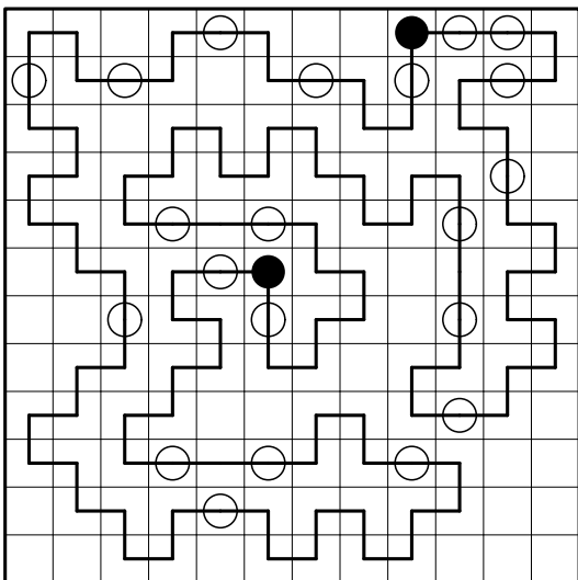
4.5 Exklusives Masyu
